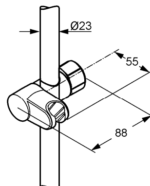
Dimensional drawing
