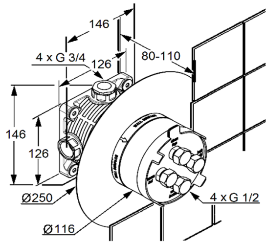
Dimensional drawing
