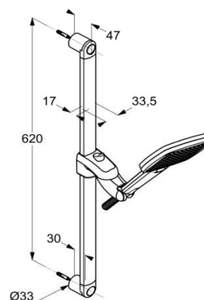
Dimensional drawing
