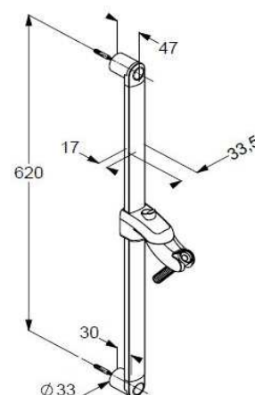
Dimensional drawing
