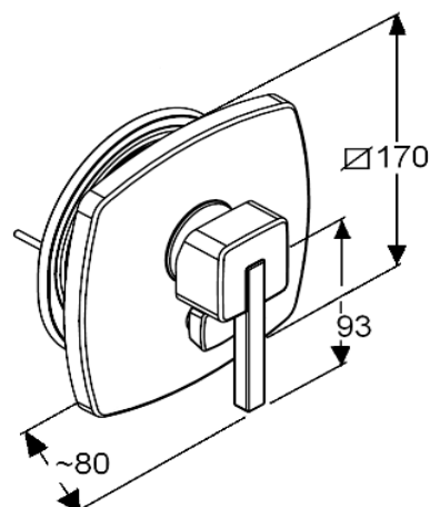
Dimensional drawing
