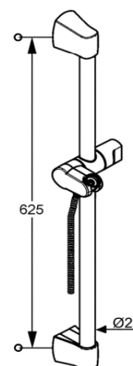
Dimensional drawing
