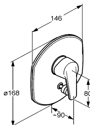
Dimensional drawing
